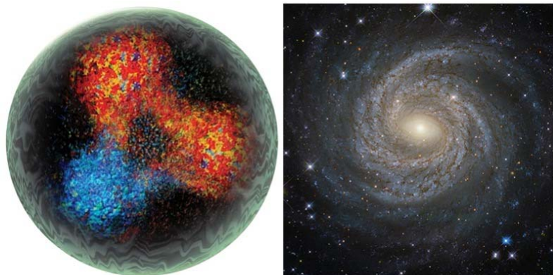
Fig. 1 The four fundamental interactions describe the behavior of matter on all scales, from the subatomic—illustrated at left in an artist's impression of the three-quark composition of the proton—to the cosmic, shown at right in a Hubble Space Telescope image of the galaxy NGC 6814. The diameter of a proton is approximately 8.7 \times 10^{-16} m, while the galaxy's diameter is approximately 8.0 \times 10^{20} m. [Credit: Jefferson Lab (left); ESA/Hubble & NASA, Acknowledgment: Judy Schmidt (Geckzilla)(right)]
