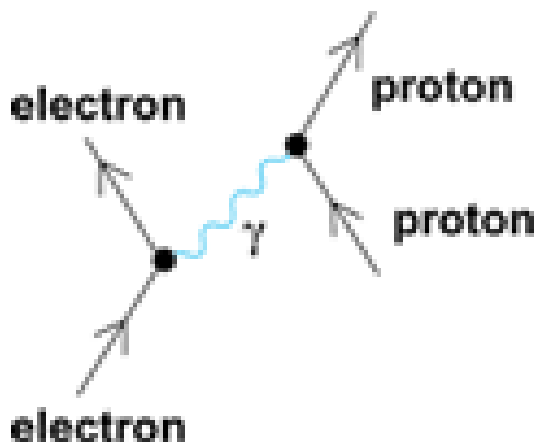
Fig. 2 Feynman diagram of electromagnetic interaction between an electron and a proton.
