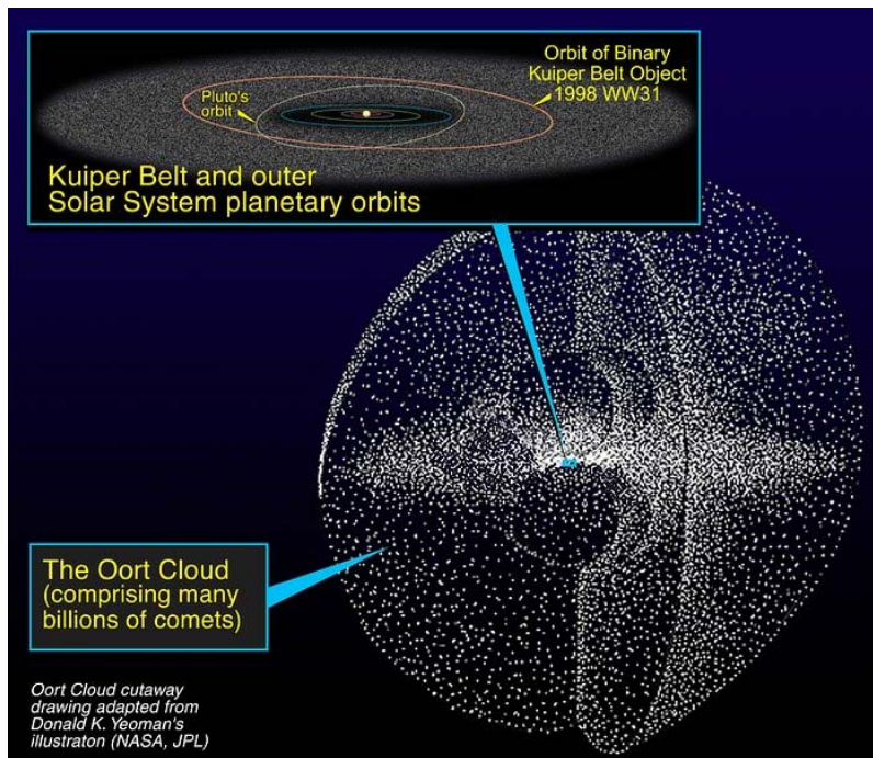
Fig. 2 Schematic of the relationship between the Kuiper Belt and Oort Cloud. The former has a disk shape (shown in the inset) that is within the encompassing shell of the Oort Cloud, consisting of billions of comets. The inset shows Pluto's orbit in relation to the outer planets, with the inner planet orbits not depicted. Also shown is the orbit of a Kuiper Belt binary object called 1998 WW31. Note: not to scale. [Credit: NASA/ESA and A. Feild (Space Telescope Science Institute)]
