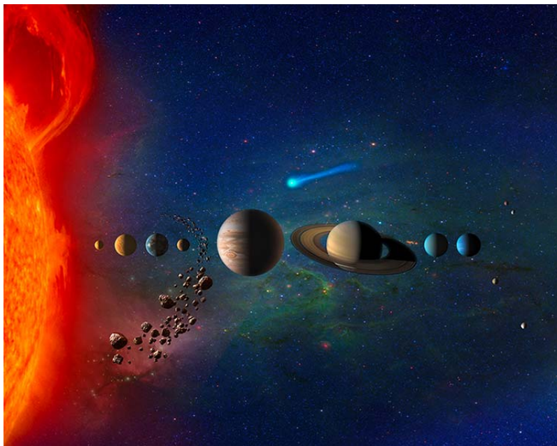
Fig. 1 An artist's impression of the main bodies and other representative objects in the solar system; note that objects are not to scale. The Sun is shown at left, with the eight planets then appearing from left to right in their proper orbital order, from nearest (Mercury) to farthest (Neptune). Also depicted is the asteroid belt between Mars and Jupiter (the fourth and fifth planets from the left, respectively). A comet is depicted above Jupiter and Saturn. Beyond Neptune at far right, several dwarf planets (such as Pluto) are shown. (Credit: NASA)
