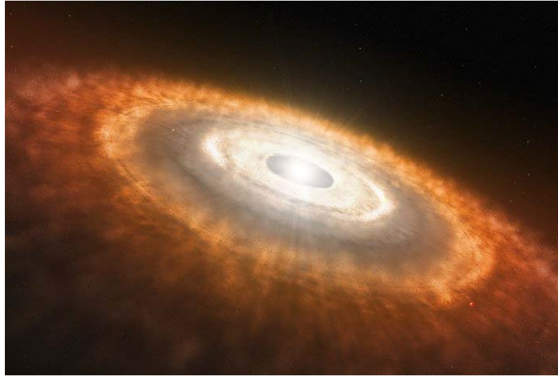
Fig. 4 An artist's impression of a protoplanetary disk, where some sizable planetary bodies have accumulated. (Credit: ESO/L. Calçada)
