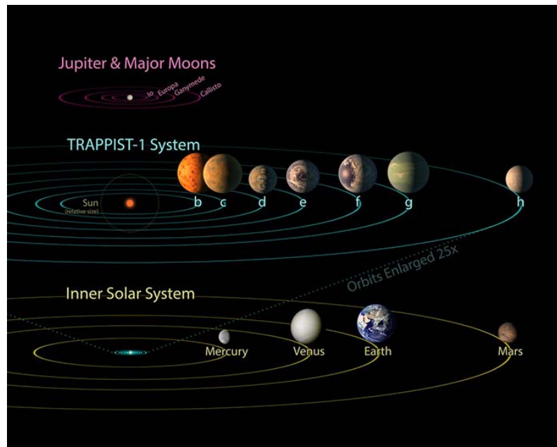
Fig. 5 A graphic comparing the TRAPPIST-1 exoplanetary solar system (middle) to our solar system (bottom) and the solar-system-in-miniature that is the planet Jupiter and its four largest moons (top). The star, TRAPPIST-1, is a small, cool, red dwarf located approximately 40 light-years from the Sun. It hosts seven terrestrial planets, all within orbits that are significantly closer to their star than Mercury is to our Sun. Because their star is cooler and dimmer than the Sun, these worlds are temperate, with some being potentially habitable. The exoplanet closest to TRAPPIST-1, designated TRAPPIST-1b, is at an approximate distance as Callisto is to Jupiter, the gas giant's outermost major moon. [Credit NASA/JPL-Caltech/R. Hurt, T. Pyle (IPAC)]
